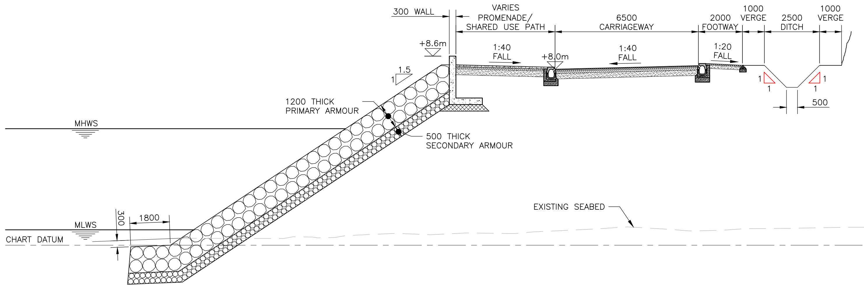
TYPICAL SECTION THROUGH ACCESS ROAD SCALE 1:100
