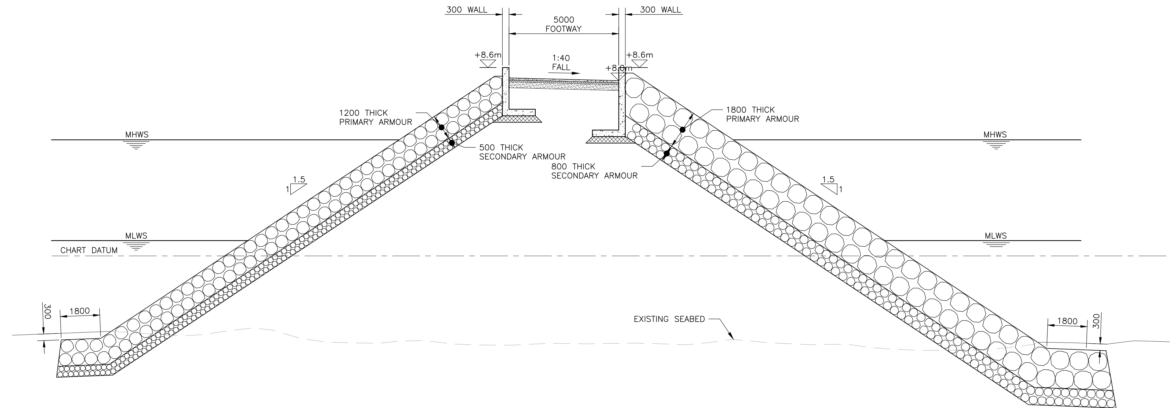
TYPICAL SECTION THROUGH BREAKWATER SCALE 1:100
